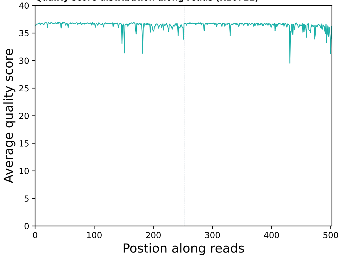
Quality score distribution along reads (R10721)
